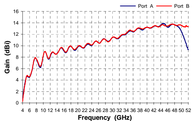
Gain
