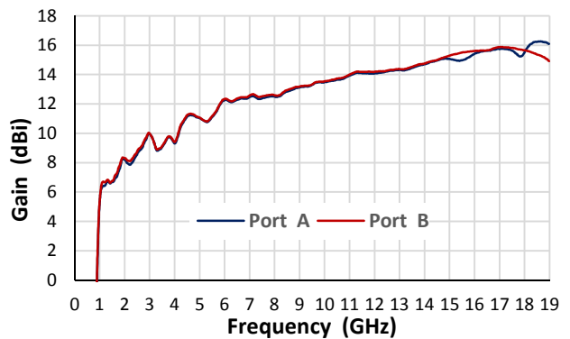
Cross Polarization
