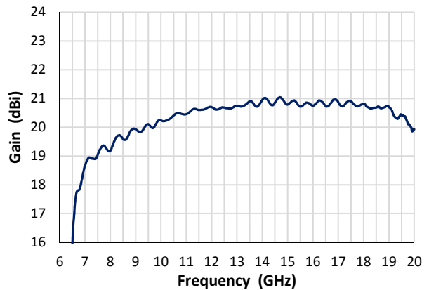
Gain
