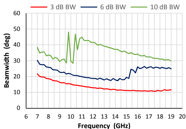
E plane
