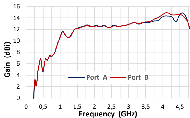
Gain
