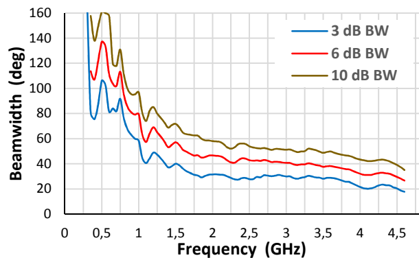
H plane
