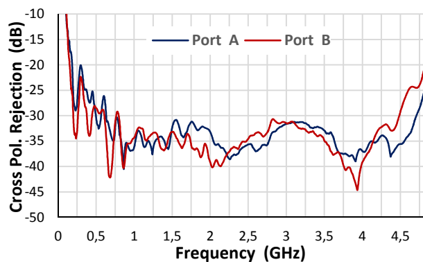
Cross Polarization
