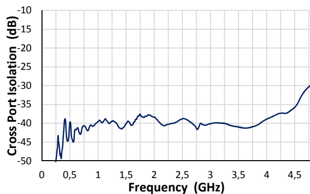
Cross Port Isolation
