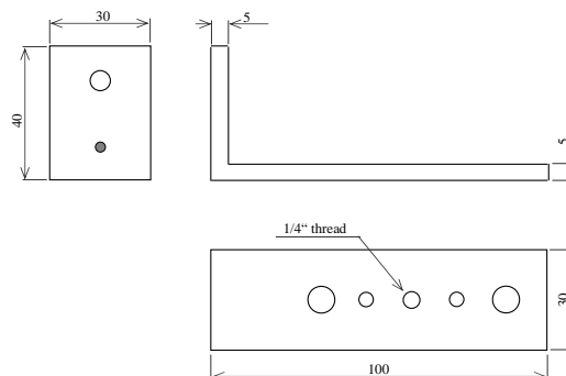
Flange / Adapter
